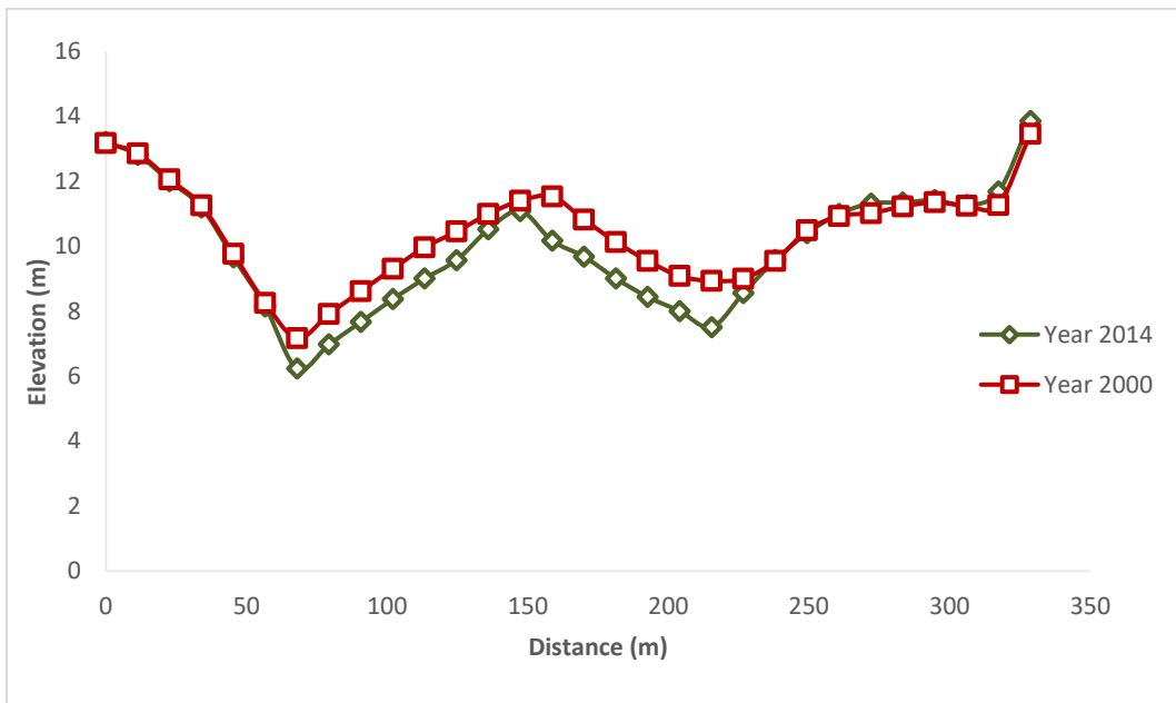
Fig. 4. 10 Cross profile of section J during 2000 and 2014
