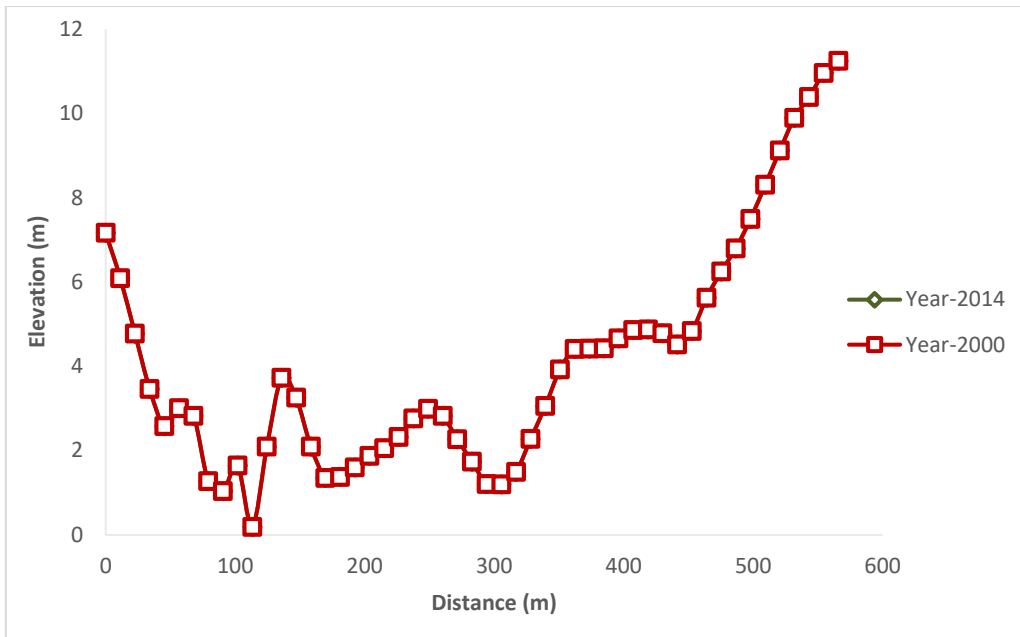
Fig. 4. 15 Cross profile of section O during 2000 and 2014
