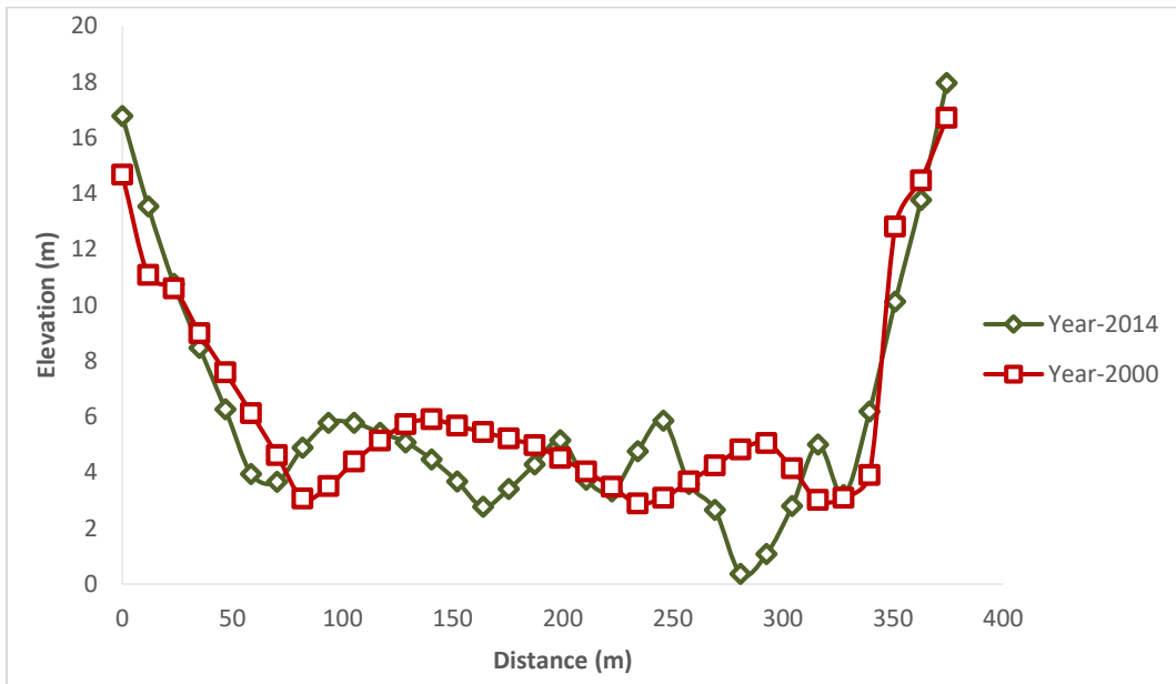
Fig. 4. 4 Cross profile of section D during 2000 and 2014
