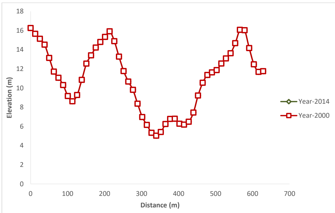
Fig. 4. 18 Cross profile of section R during 2000 and 2014
