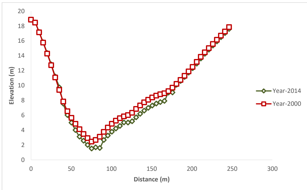
Fig. 4. 9 Cross profile of section I during 2000 and 2014
