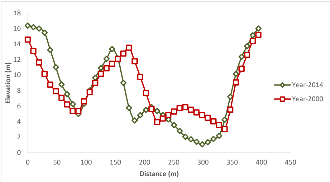
Fig. 4. 3 Cross profile of section C during 2000 and 2014
