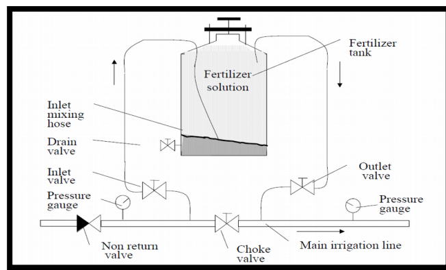
Fig. 2.3 Fertilizer tank Source: (Imas, 1999)
