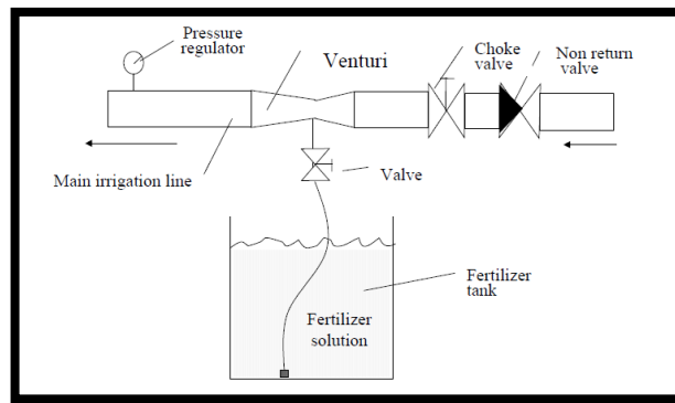
Fig. 2.1 Ventury injector
