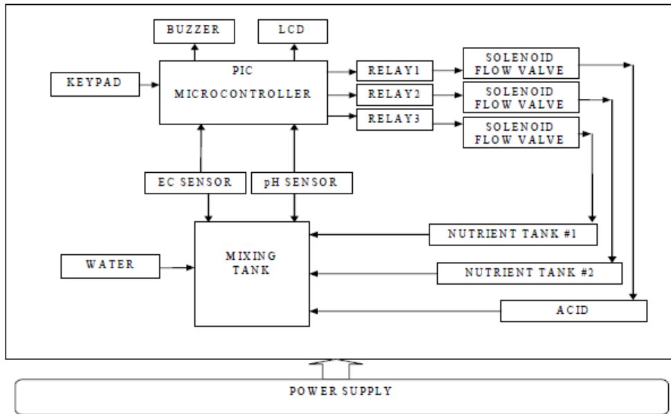
Fig. 2.4 Fertilization control system
