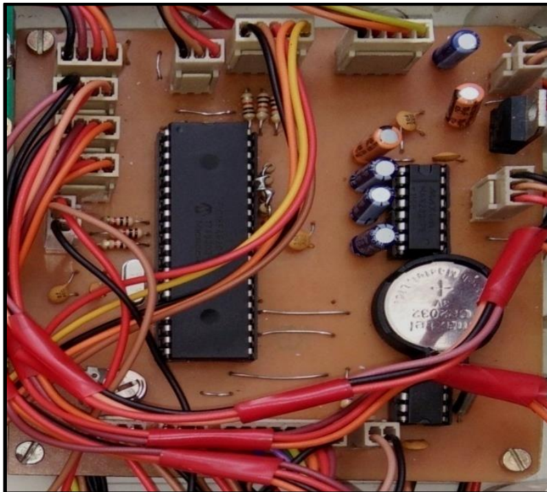
Plate 2. Board with microcontroller
