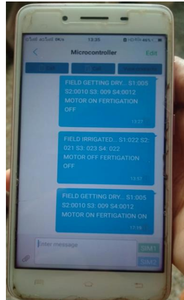
Fig. 21. Status message from the system before irrigation
