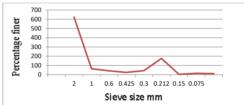
Fig. 12 Sieve analysis of Laterite soil
