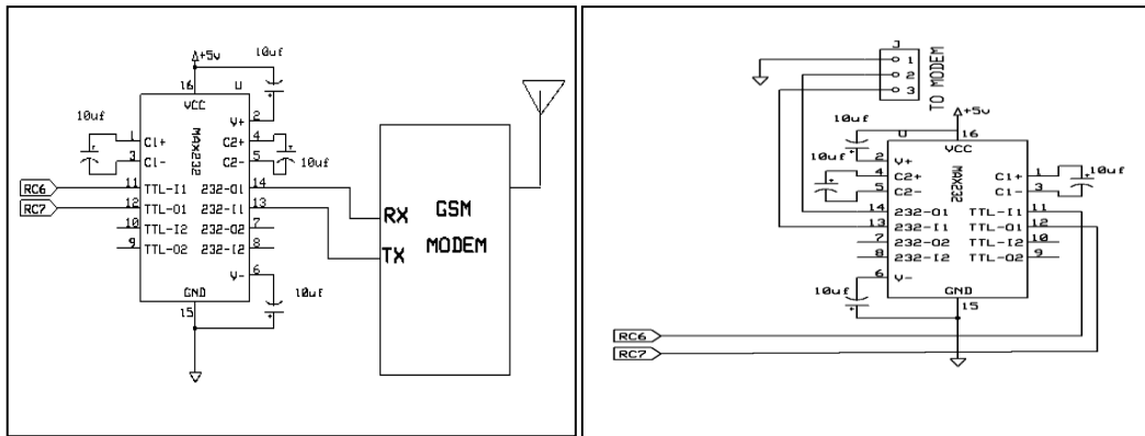
Fig.9. Circuit of GSM modems
