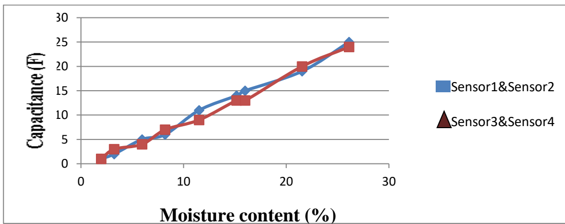
Fig. 19. Calibration curves of capacitance sensors in black soil
