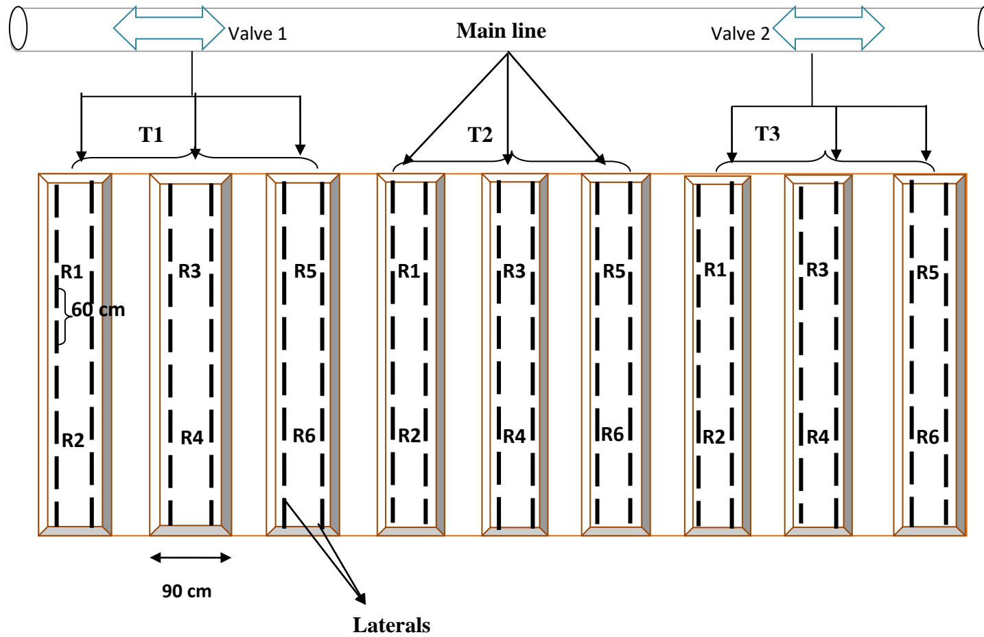
Fig 11. Field layout
