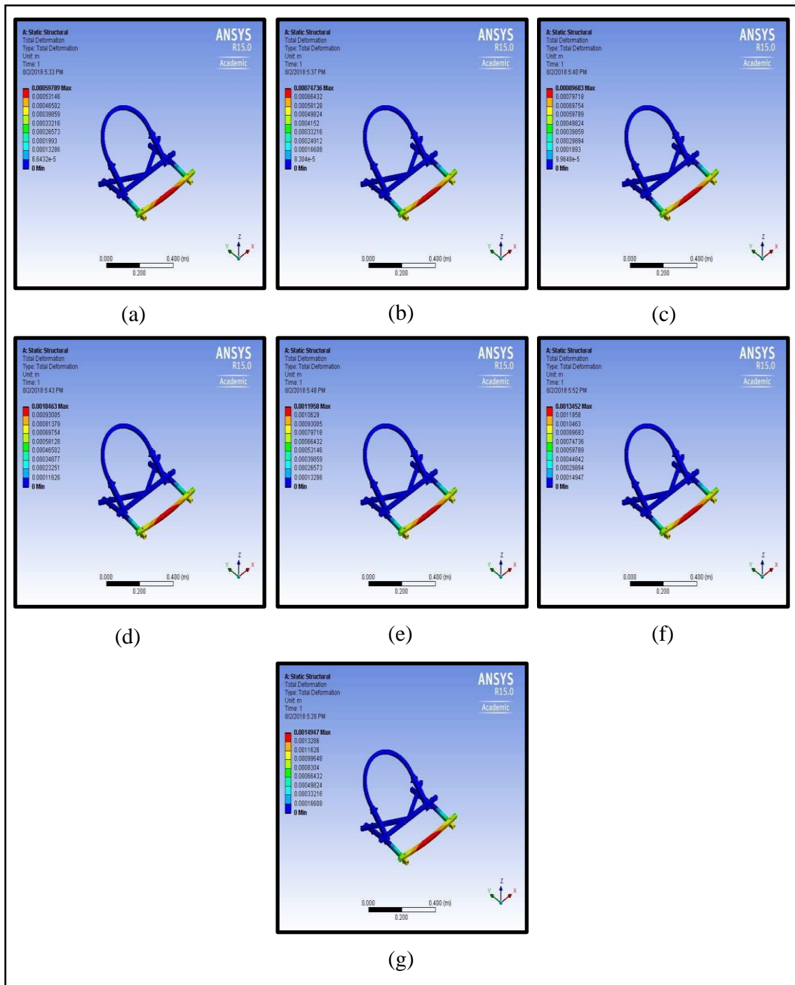
Plate 4.6 Total deformation of the bottom frame of KAU coconut palm climber at loads of a) 400 N, (b) 500 N, (c) 600 N, (d) 700 N, (e) 800 N, (f) 900 N and (g) 1000N
