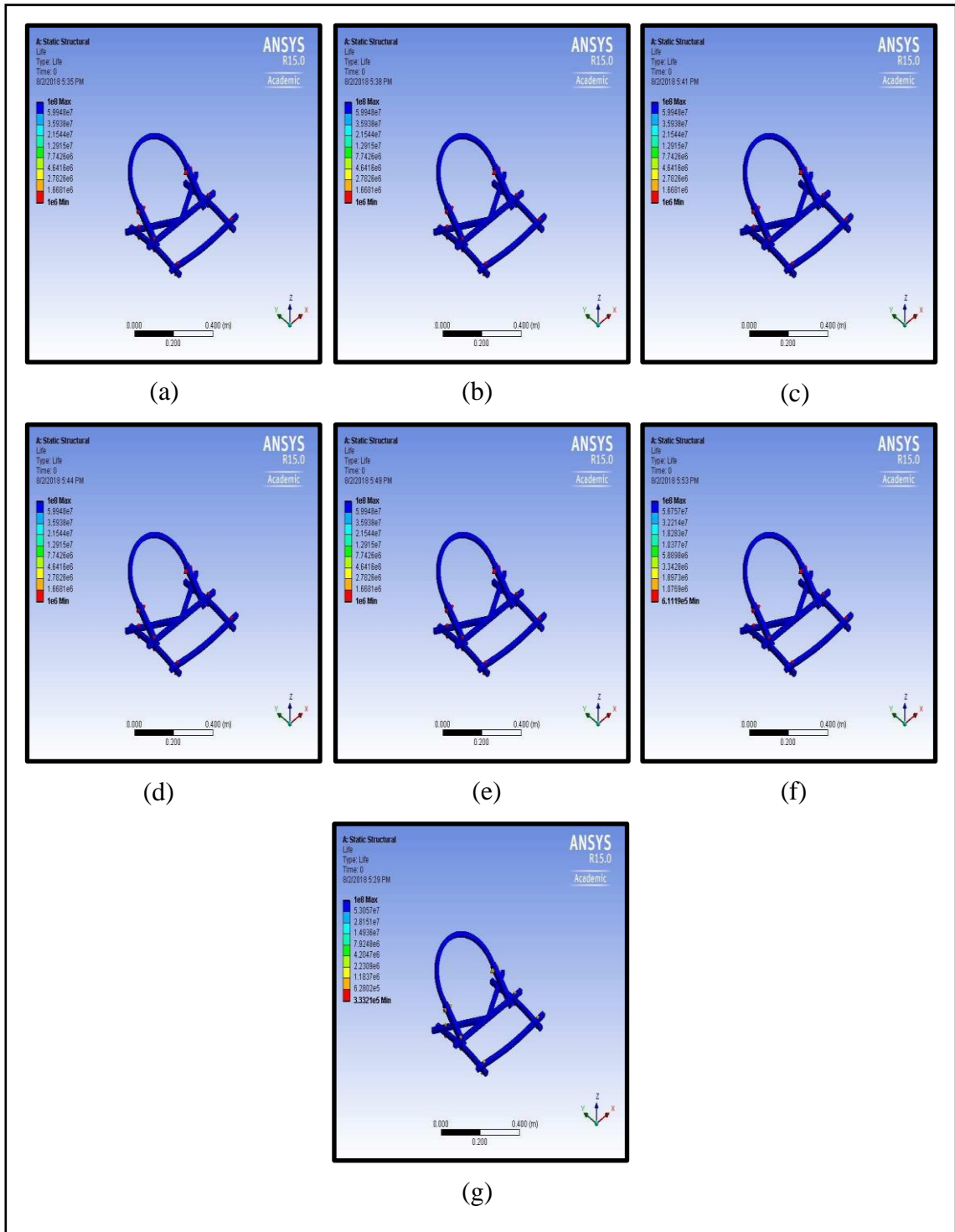
Plate 4.9 Fatigue life of the bottom frame of KAU model at loads of (a) 400 N, (b) 500 N, (c) 600 N, (d) 700 N, (e) 800 N, (f) 900 N and (g) 1000N
