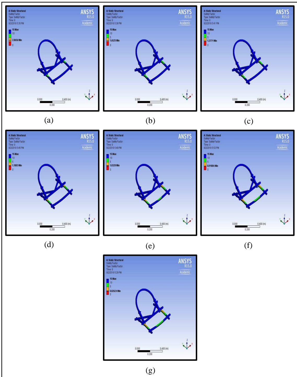
Plate 4.10 Factor of safety of the bottom frame of KAU model at loads of (a) 400 N, (b) 500 N, (c) 600 N, (d) 700 N, (e) 800 N, (f) 900 N and (g) 1000N
