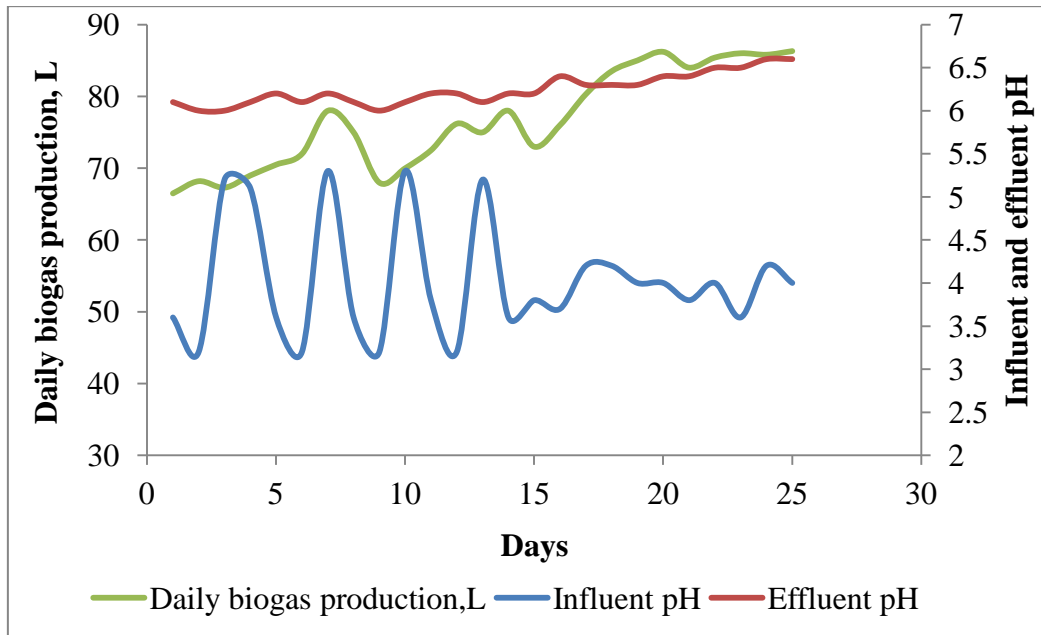
Fig. 4.12 Variation of pH and daily biogas production during 12-day HRT
