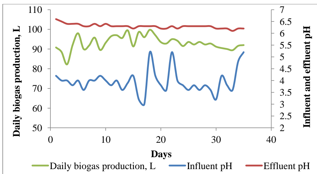
Fig.4.13 Variation of pH and daily biogas production during 10-day HRT
