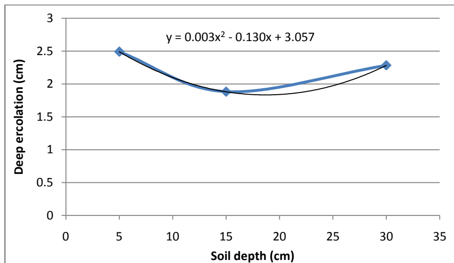
Figure 4.19 Regression curve for deep percolation (10 cm lateral)
