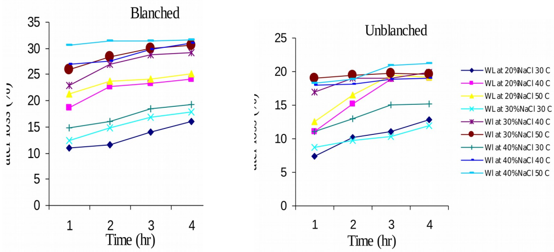
Fig.4.2 Effect of solute concentration on water loss for blanched and unblanched karimunda variety
