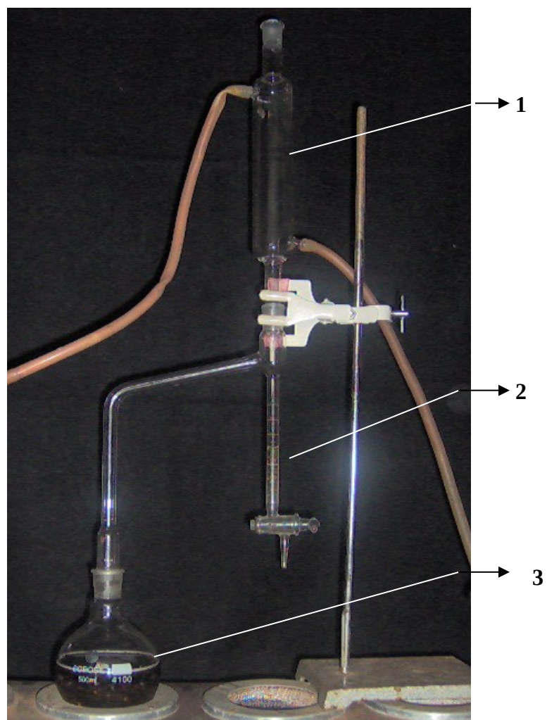
Plate 3.5 Clevenger apparatus
