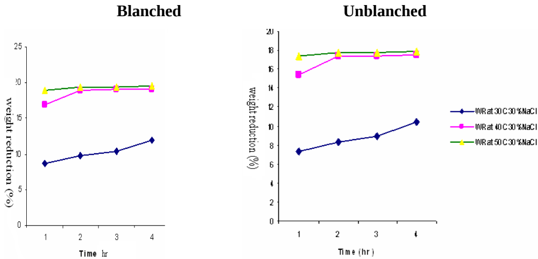
Fig.4.11 Effect of time on weight reduction for blanched and unblanched Panniyr variety
