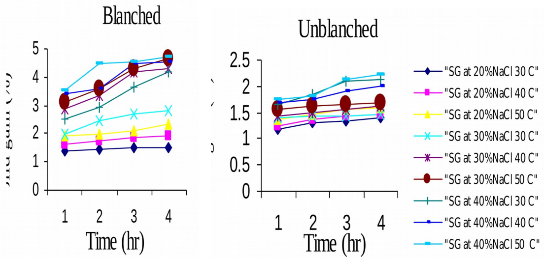
Fig.4.4 Effect of solute concentration on solid gain for blended and unblended samples of Karimunda variety
