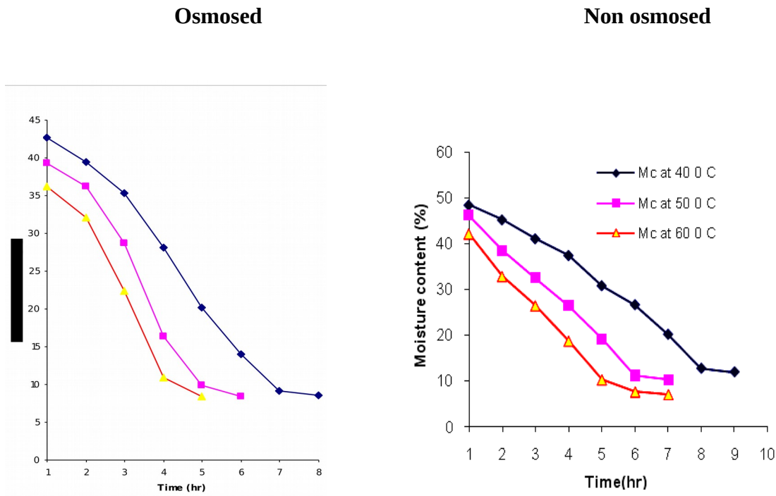
Fig.4.12 Hot air drying of osmosed and non osmosed samples
