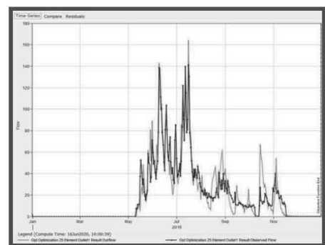
Fig. 6. Simulated and observed hydrograph during calibration period
