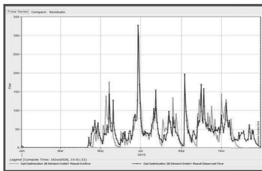
Fig. 6. Simulated and observed hydrograph during calibration period
