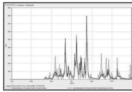
Fig. 7. Simulated and observed hydrograph during validation period
