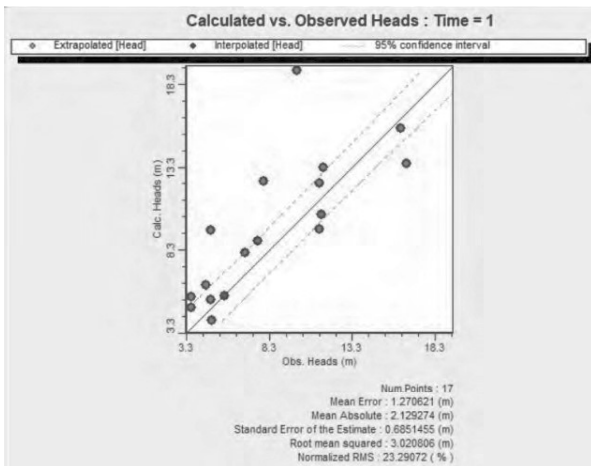
Fig. 7. Computed vs. observed water levels after validation
