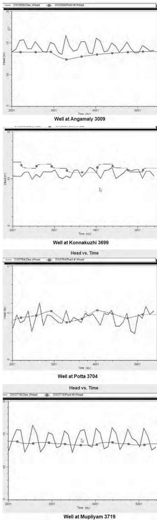
Fig. 5. Computed and observed head vs time graph of selected wells after calibration
