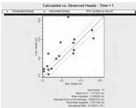
Fig. 2. Observed vs. computed water levels after steady-state calibration
