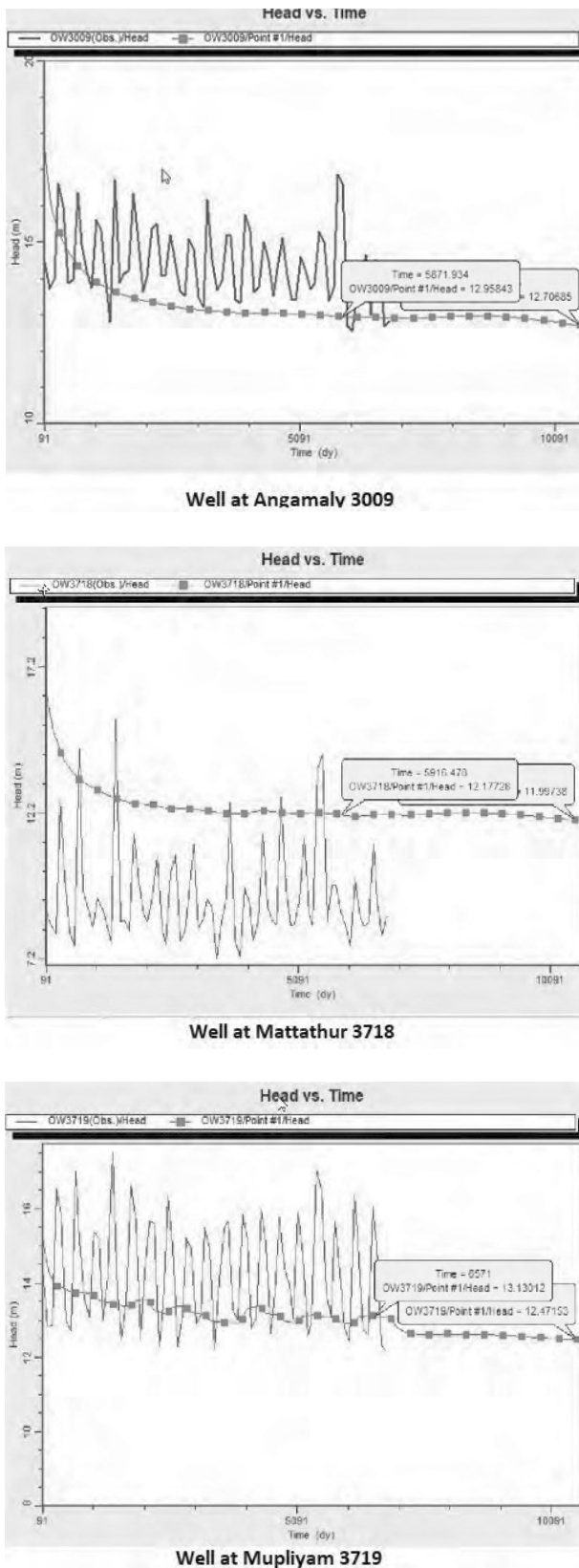
Fig. 11. Scenario II - Predicted water levels of selected wells after 10 years from the end of the validation period
