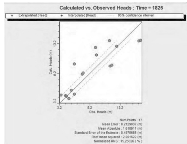
Fig. 3. Observed vs. computed water levels on 1826th day of the calibration period
