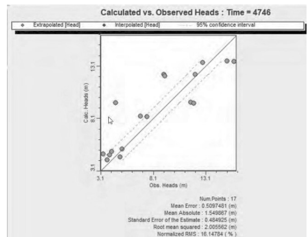
Fig. 4. Observed vs. computed water levels on 4746th day of the calibration period
