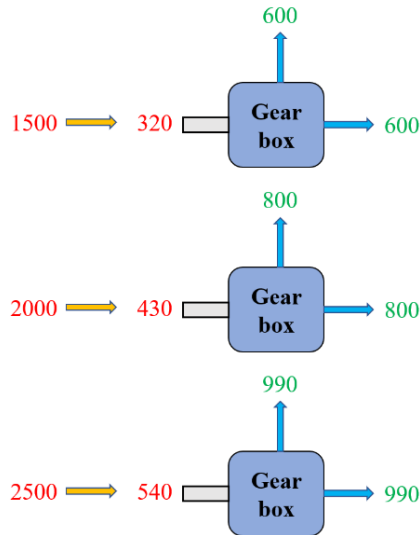
Fig. 3.27 Variation in gearbox output speeds, RPM
