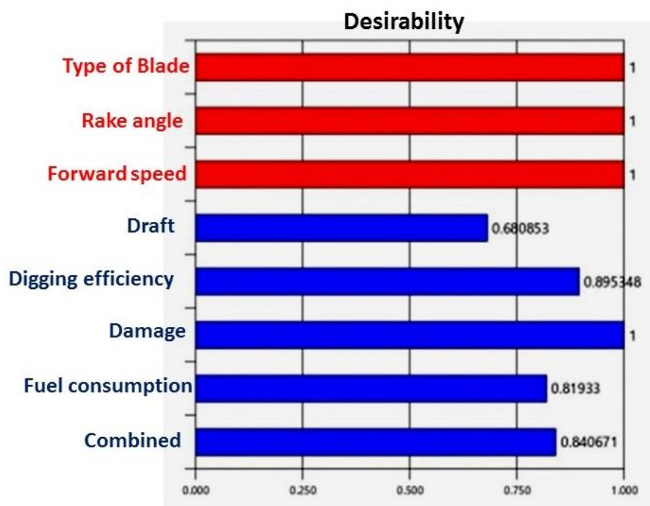
Fig 4.31 Desirability index for optimized digging unit for ginger
